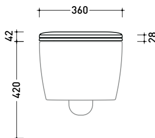
art. PY118S - PY117S - PY117RS vista frontale / front view
