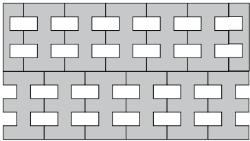
laying scheme 3 35 pcs / sqm
